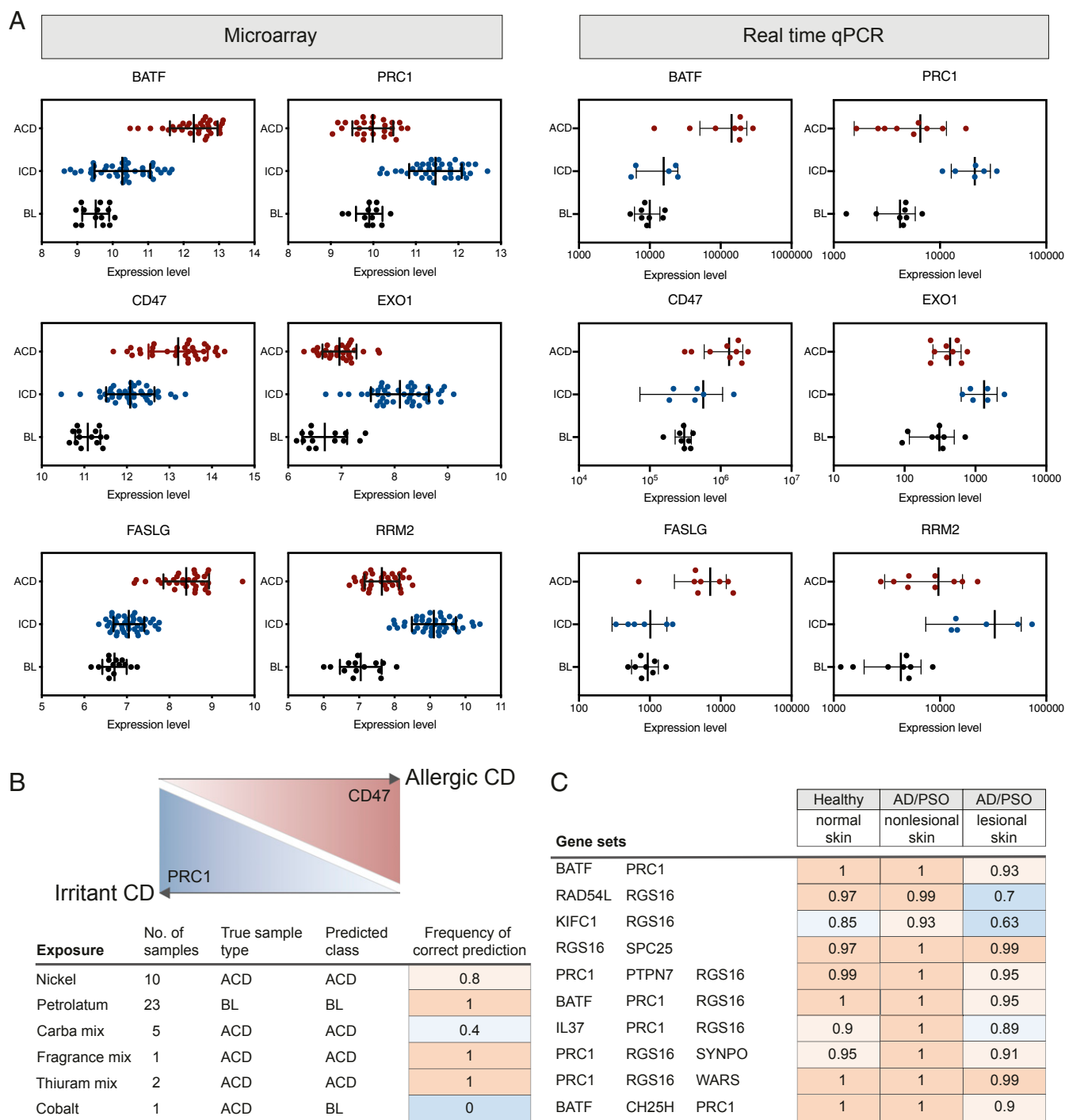
Fig. 5. Validation of biomarkers selected by GARBO. (A) Expression levels of selected biomarkers measured by arrays (panels on the Left ) and validated by real time qPCR in an independent group of patients (panels on the Right ). Error bars correspond to SD. Selected combinations of biomarkers were tested in external datasets of (B) ACD (access code GSE60028) and (C) atopic dermatitis (AD) and psoriasis (PSO) (access code E-MTAB-8149), revealing predictive potential of the biomarkers, reported as the frequency of correct prediction. GSE60028 was used to demonstrate the generalizability of the selected biomarker models on new, external ACD samples; the second external testing dataset (E-MTAB-8149) aimed to prove the uncertainty of the biomarker models when trying to classify lesional and nonlesional skin in psoriasis and atopic dermatitis.
